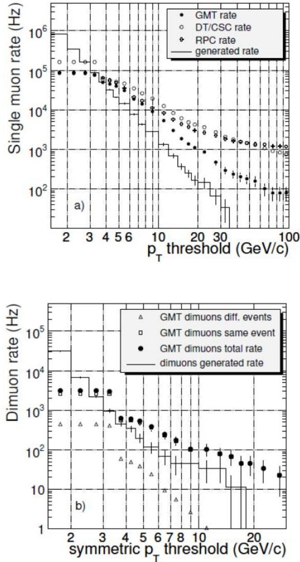
Figure 3.14: Level-1 trigger rate at \mathcal{L} = 2 \times 10^{33} \text{ cm}^{-2}\text{s}^{-1} as a function of p_T threshold for single- (top) and di-muon trigger (bottom), at generator level (histogram) and from the Global Muon Trigger (dark circles with error bars). The single-muon rate plot also shows trigger rates that would occur if the RPC system or the combined DT/CSC system were operated standalone (crosses and open circles). The di-muon rate plot shows separately the contributions from the same (squares) and different (triangles) p-p collisions within one BX [3].
