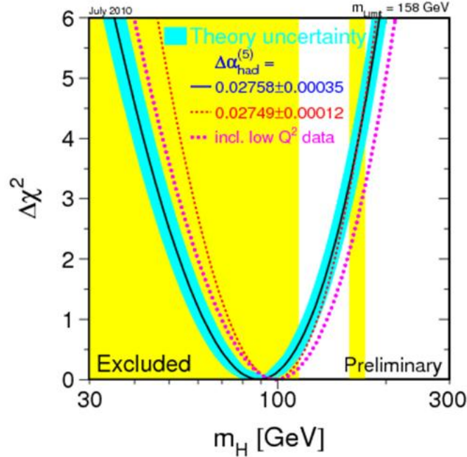
Figure 1.2: \Delta\chi^2 curve obtained from high- Q^2 precision electroweak measurements, performed at LEP and by SLD, CDF, and D\theta , as a function of the Higgs boson mass, assuming the Standard Model to be the correct theory of nature [22]
