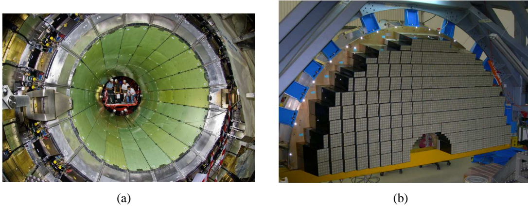
Figure 2.15: (a) The barrel positioned inside the hadron calorimeter. (b) An endcap Dee, fully equipped with supercrystals
