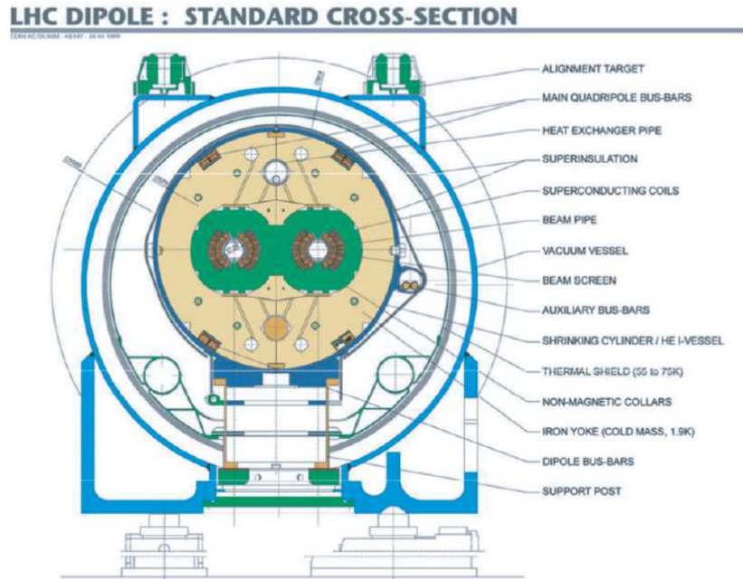
Figure 2.5: Dipole cross-section.
