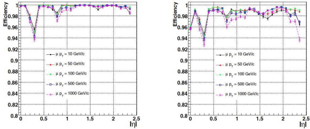
Figure 2.19: Muon reconstruction efficiency as a function of pseudorapidity for different values of p_T . Left panel: standalone reconstruction (using only hits from the muon system with a vertex constraint). Right panel: global reconstruction (using hits from both the muon system and the tracker).
