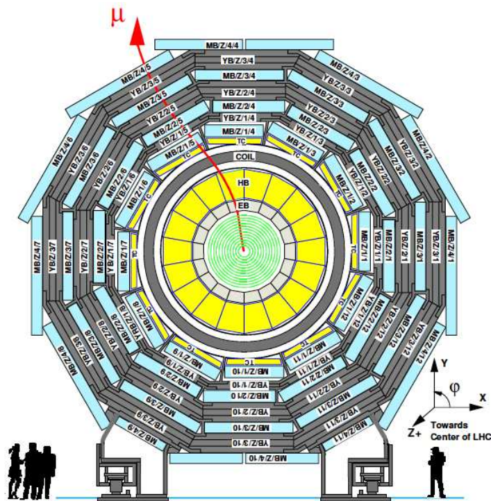
Figure 2.21: Layout of the CMS barrel muon DT chambers in one of the 5 wheels. The chambers in each wheel are identical with the exception of wheels -1 and +1 where the presence of cryogenic chimneys for the magnet shortens the chambers in 2 sectors.
