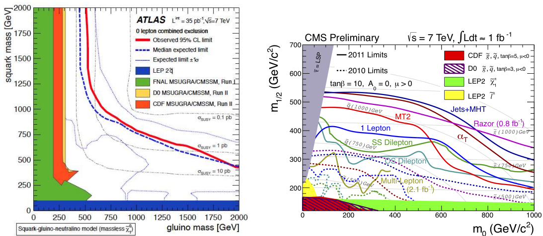
Figure 3.10: 95% C.L. exclusion limits in the (gluino, squark) mass plane for ATLAS experiment (a) and in the ( m_0, m_{1/2} ) mass plane for CMS experiment (b). m_0 and m_{1/2} are the masses of the superparticles with spin 0 and 1/2, respectively.
