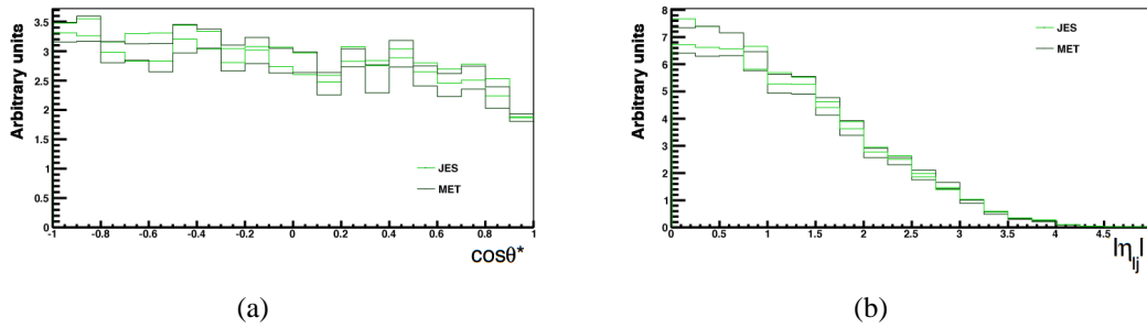
Figure 5.25: JES (varied by \pm 3.5\% ) and E_T ('clustered' varied by the same factor as JES , summed in quadrature with 'unclustered' E_T variation of \pm 10\% ) uncertainties effect on the overall background \cos\theta_{l_j}^* and \eta_{l_j} distributions.
