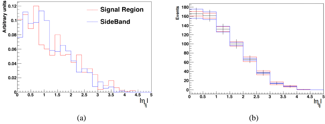
Figure 6.14: (a) Shape comparison of \eta_{lj} variable for the W/Z + X in the Signal Region vs Sideband region. (b) Effect of varying the t -channel yield (red line) by \pm 100\% and t\bar{t} yield (blue line) by \pm 10\% in the Sideband Region on the data-driven extracted shape (black line).
