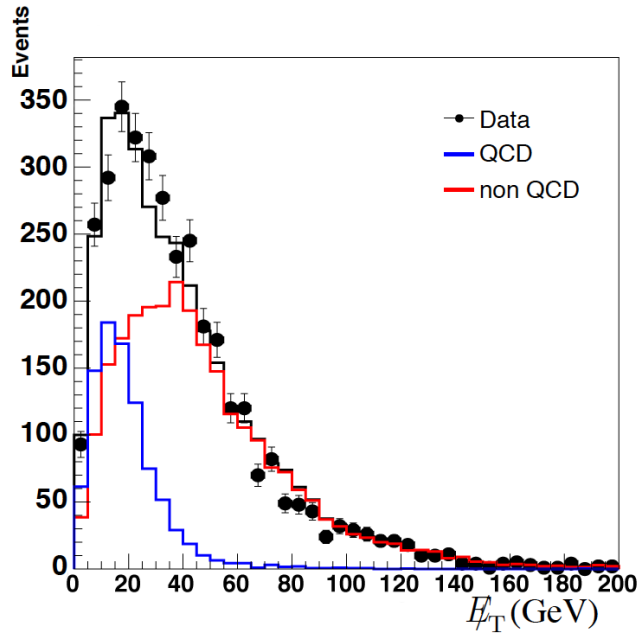
Figure 6.11: E_T fit for QCD estimation in the 2-Jet 1-Tag (signal) sample.
