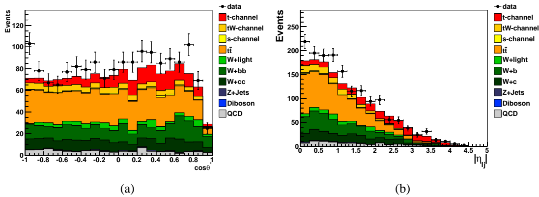
Figure 6.15: Cosine of the angle between charged lepton and untagged jet ( \cos \theta_{l_j}^* ), in the reconstructed top rest frame after the full event selection (a) and pseudorapidity of the untagged jet ( \eta_{l_j} ) after the full event selection.
