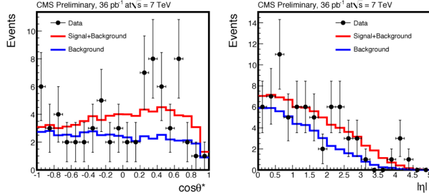
Figure 5.20: Fit to \cos \theta_{ij}^* and \eta_{ij} .
