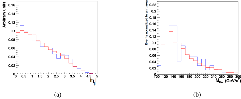
Figure 6.13: \eta_j (a) and M_{bl\nu} (b) distributions for Monte Carlo QCD samples obtained after an anti isolation and ID cut (red) and after the standard isolation cut (blue).
