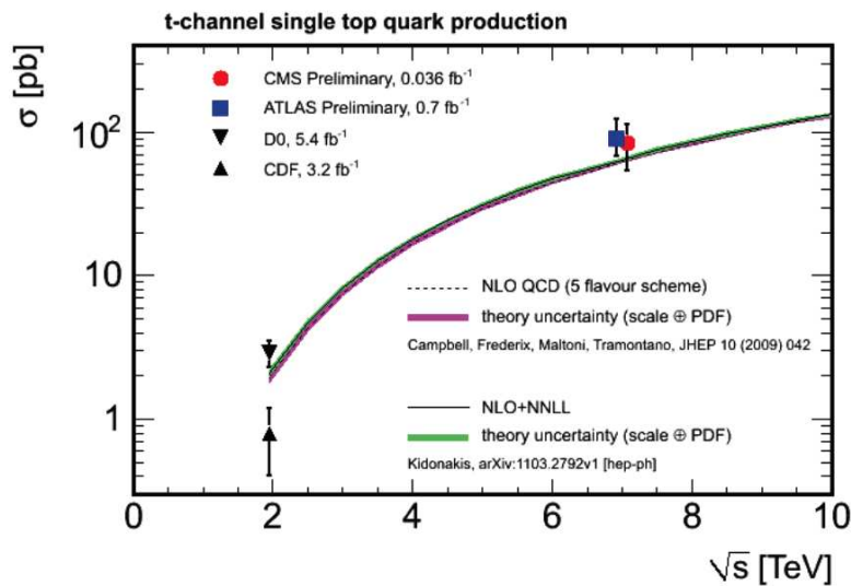
Figure 4.12: Single top t -channel production cross sections as measured by Tevatron and LHC and NLO,NNLL theoretical predictions.
