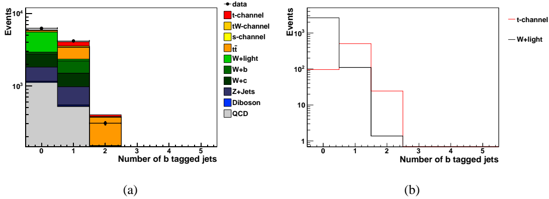
Figure 6.3: Number of jets for D_{TCHP} > 3.41 for data and simulation and for signal and W + \text{light} parts only, after the 2 jets request.
