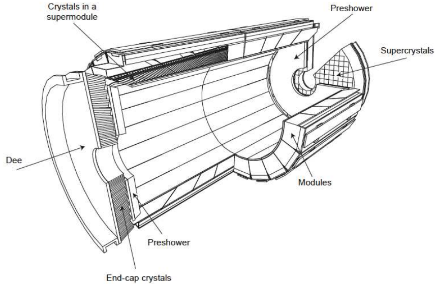
Figure 2.14: Layout of the CMS electromagnetic calorimeter showing the arrangement of crystal modules, supermodules and endcaps, with the preshower in front.
